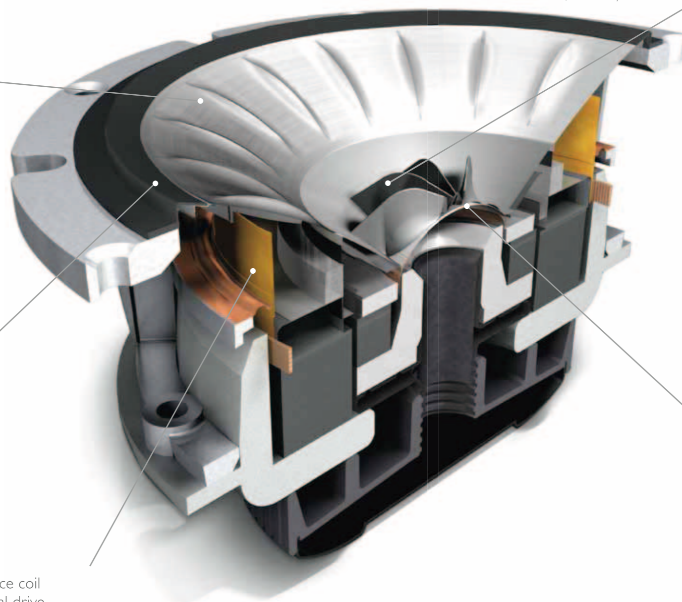
The Uni-Q driver array
