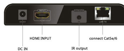
LKV373MATRIX-TX
