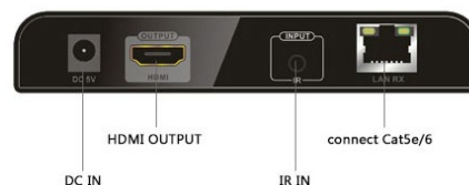
LKV373MATRIX-RX
